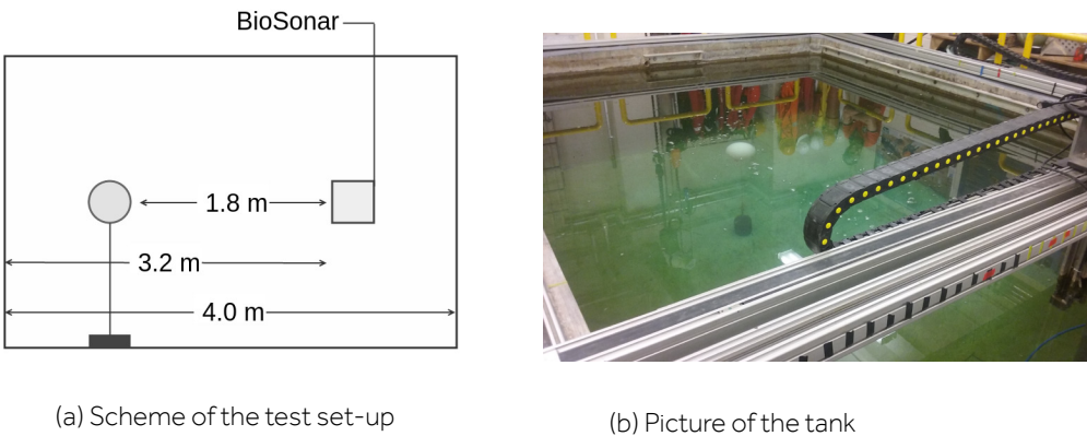
Figure 2: Test set-up
