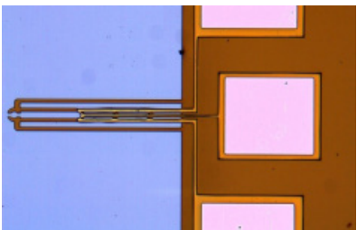
Fig. 1 An SU-8 based eletrothermal microgripper before released from substrate (IMT, Romania).
