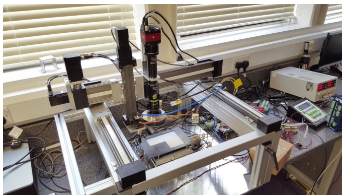
Figure 1. Hybrid micro-assembly system
