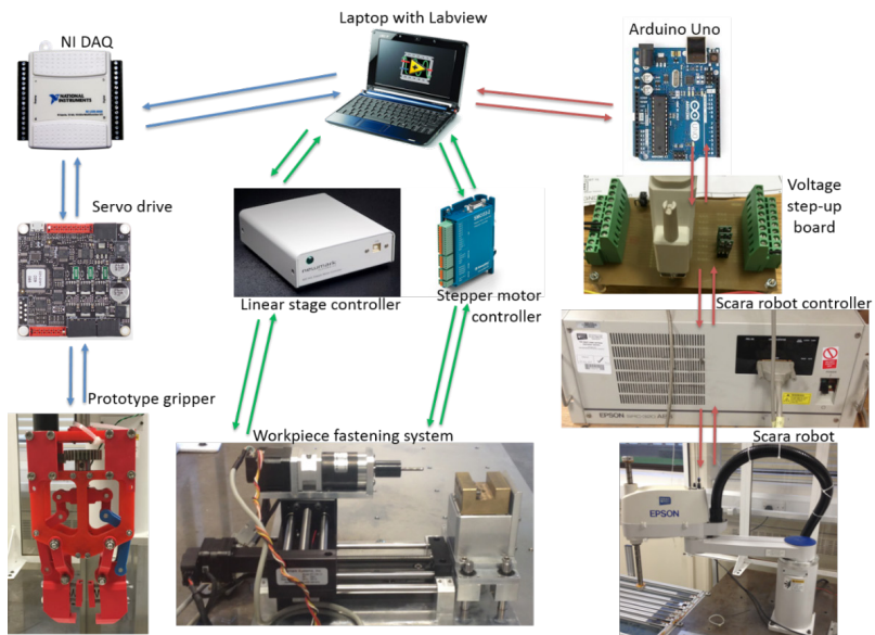
Figure 1: Component parts of the handling system and schematic diagram of their integration
