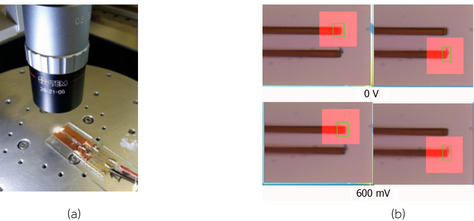
Fig. 3 (a) Setup for gripper characterisation, (b) Image tracking method for gripper displacement measurements
