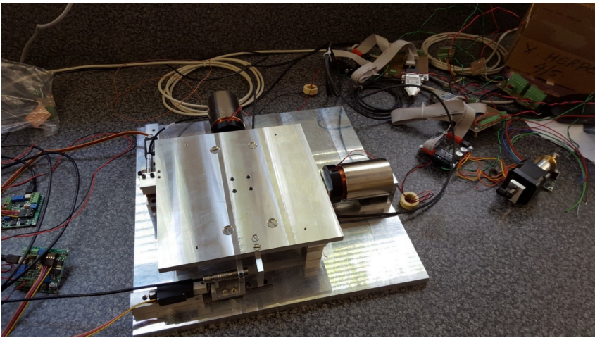
Figure 2. Micro-motion XY stage
