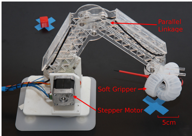
Our hard-soft hybrid arm
